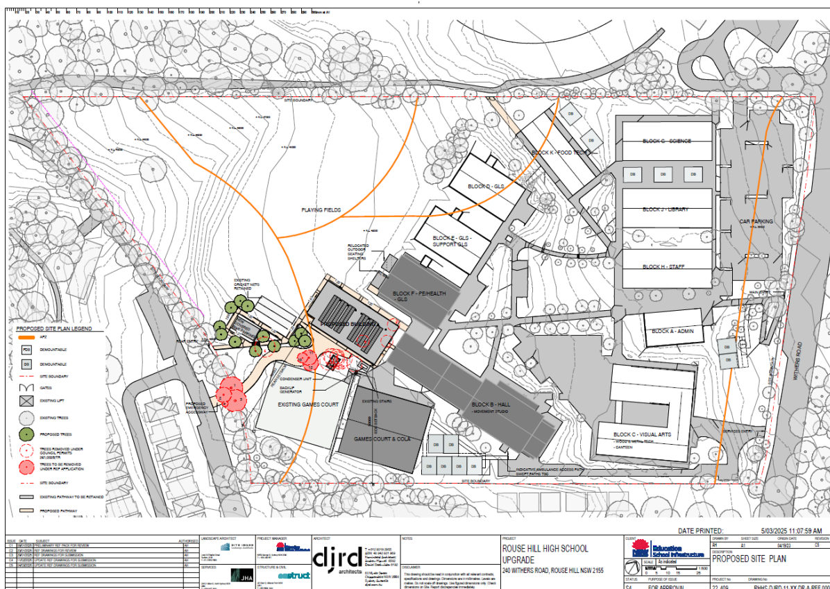
Figure 3: Rouse Hill High School Upgrade Concept Plan
